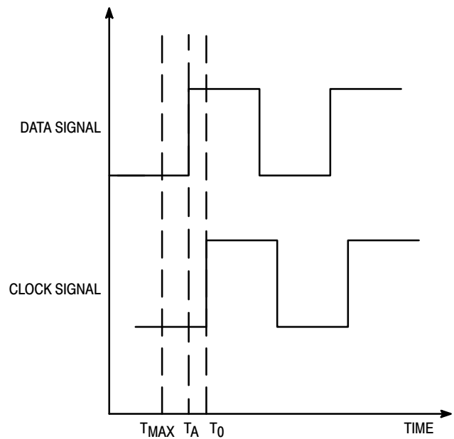
Figure 7(b) Violation of Set-Up and Hold Times
