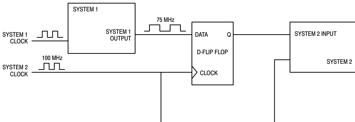
Fig. 11 System Example
