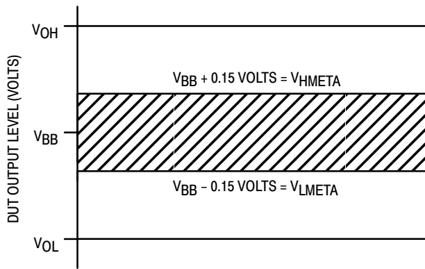
Figure 9. Output Response Defining the Metastable Region
