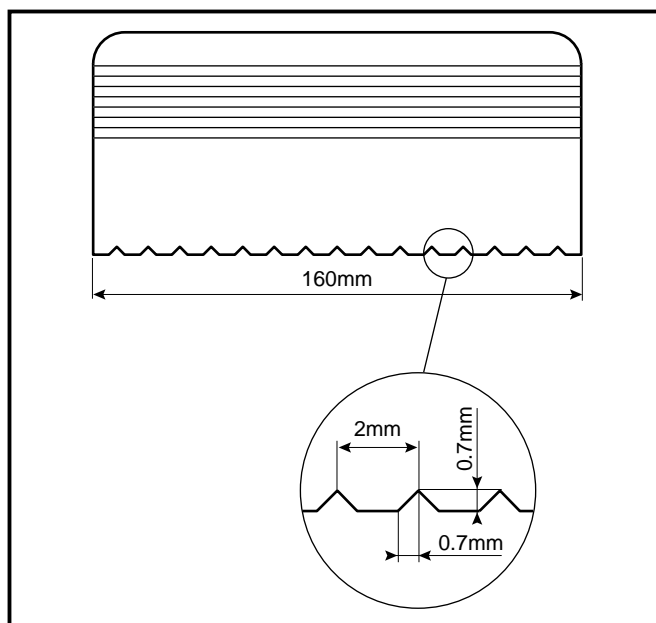
Fig. 5 Spatula profile
