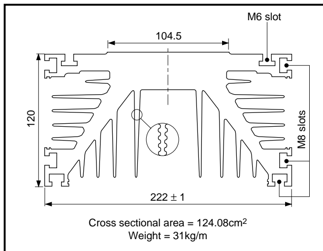
Fig. 4 Typical air cooled heatsink outline
