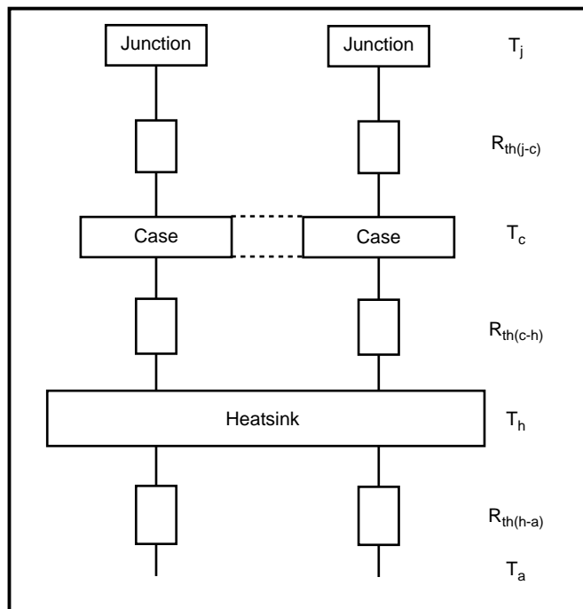
Fig. 8 Paralleling considerations
