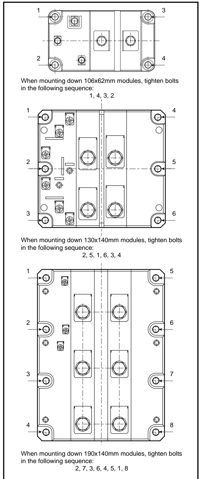
Fig. 6 Screw/bolt tightening sequence for Dynex Semiconductor IGBT modules
